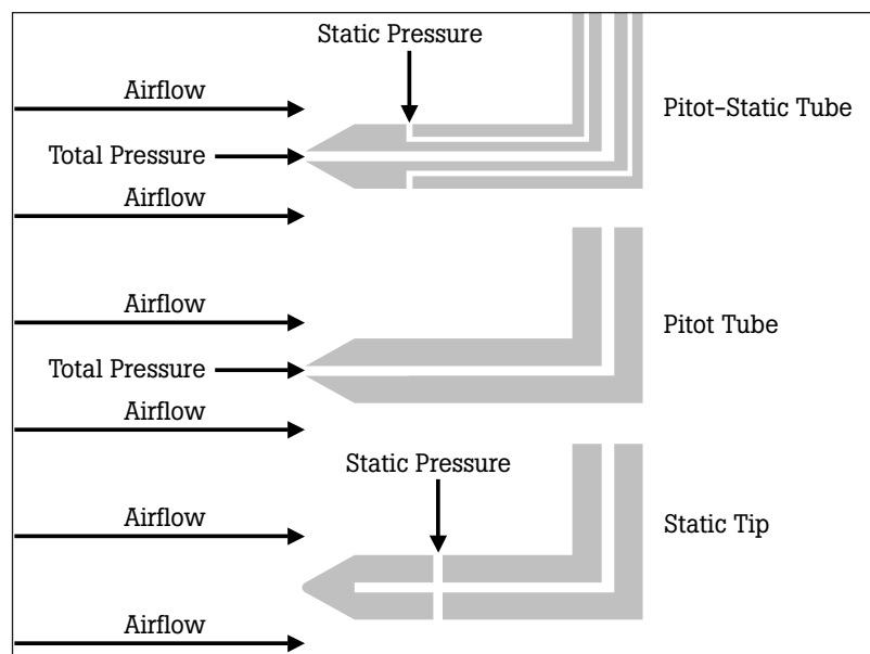
Options for sensing probes and fittings when accessing pressure measurement points.
